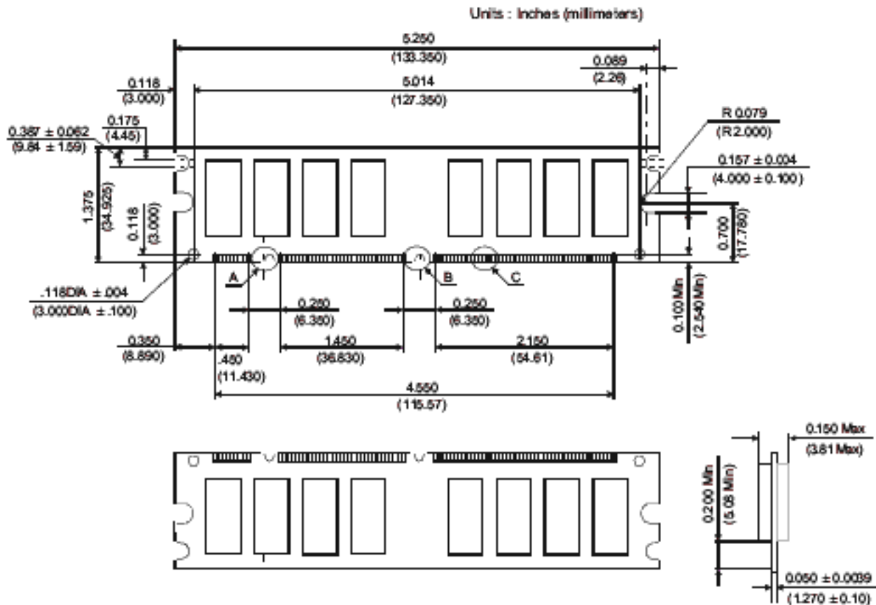
Figure 1: KVR133X64C2/512 168-Pin SDRAM Module
